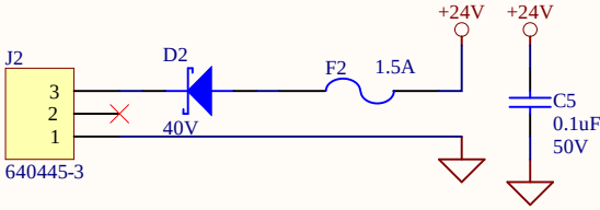
i.MX 6 Board Power Connector
